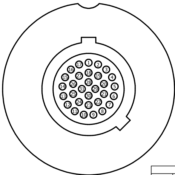
FACE VIEW
