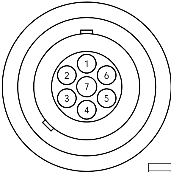
FACE VIEW
