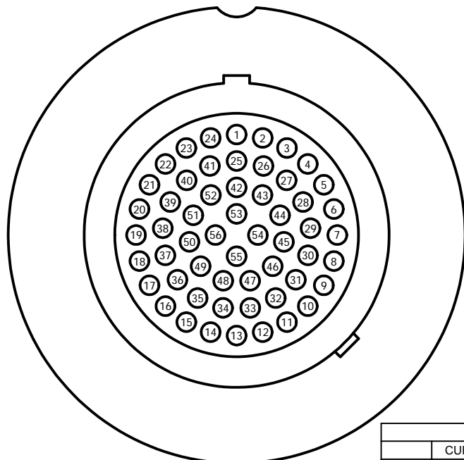
FACE VIEW
