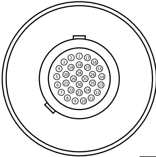
FACE VIEW
