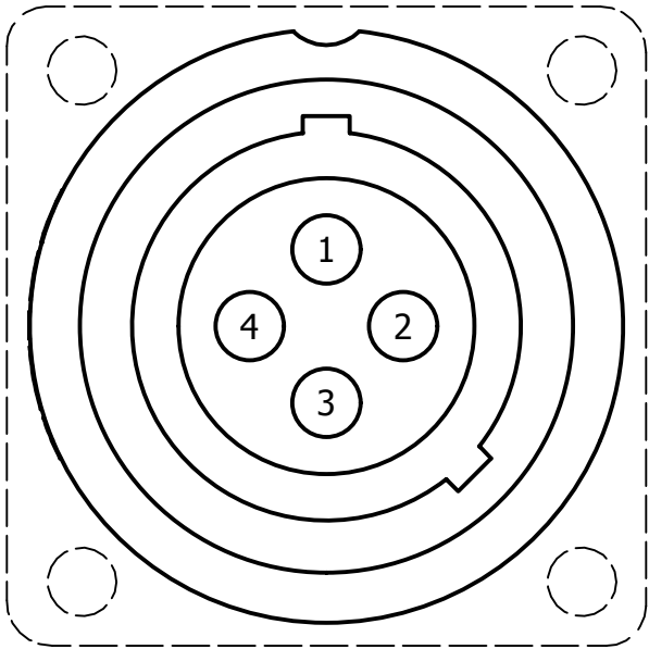
FACE VIEW
